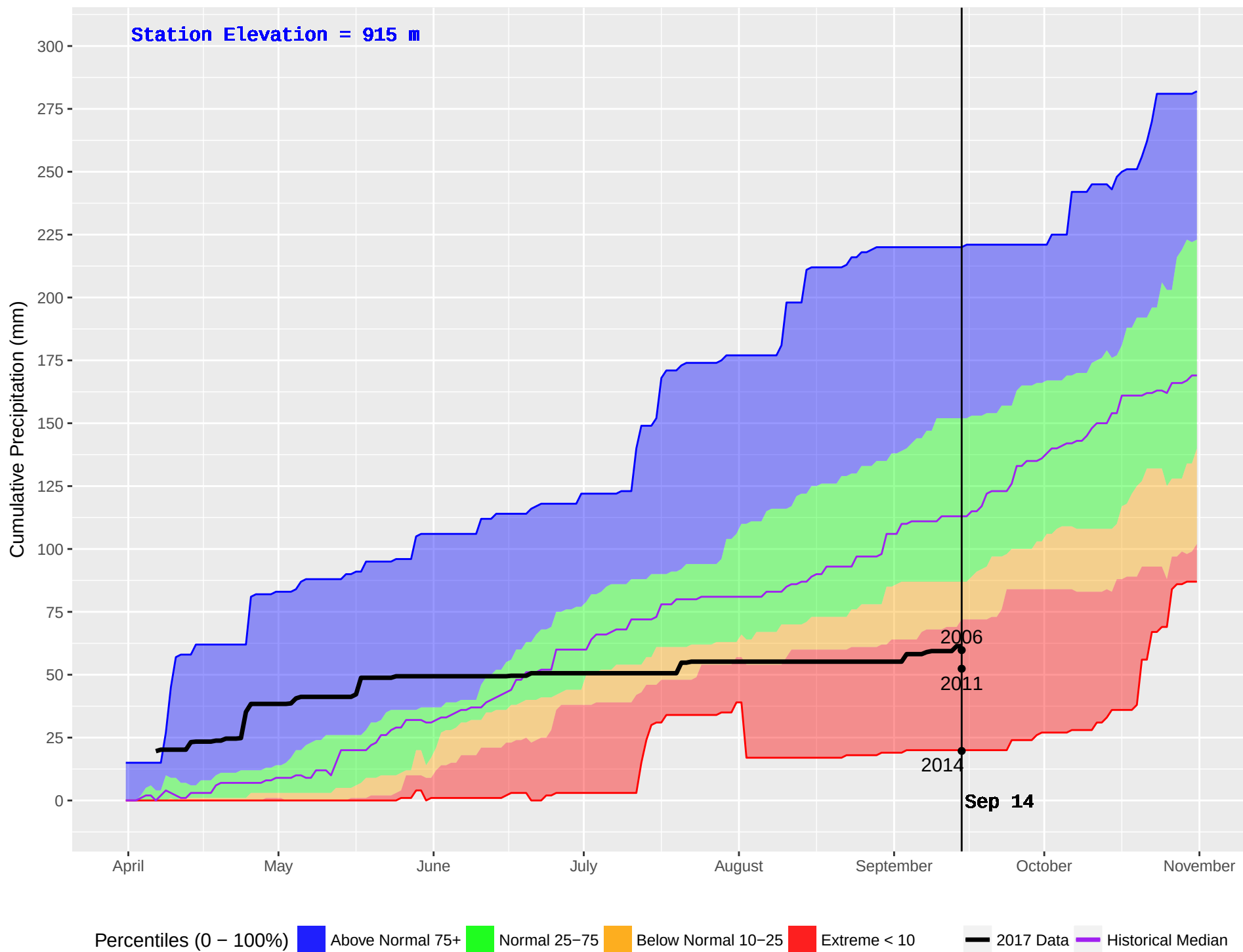
MIDDLE LAKE (226) : Historical (1989–2016) and Current (2017) Noon Cumulative Precipitation
