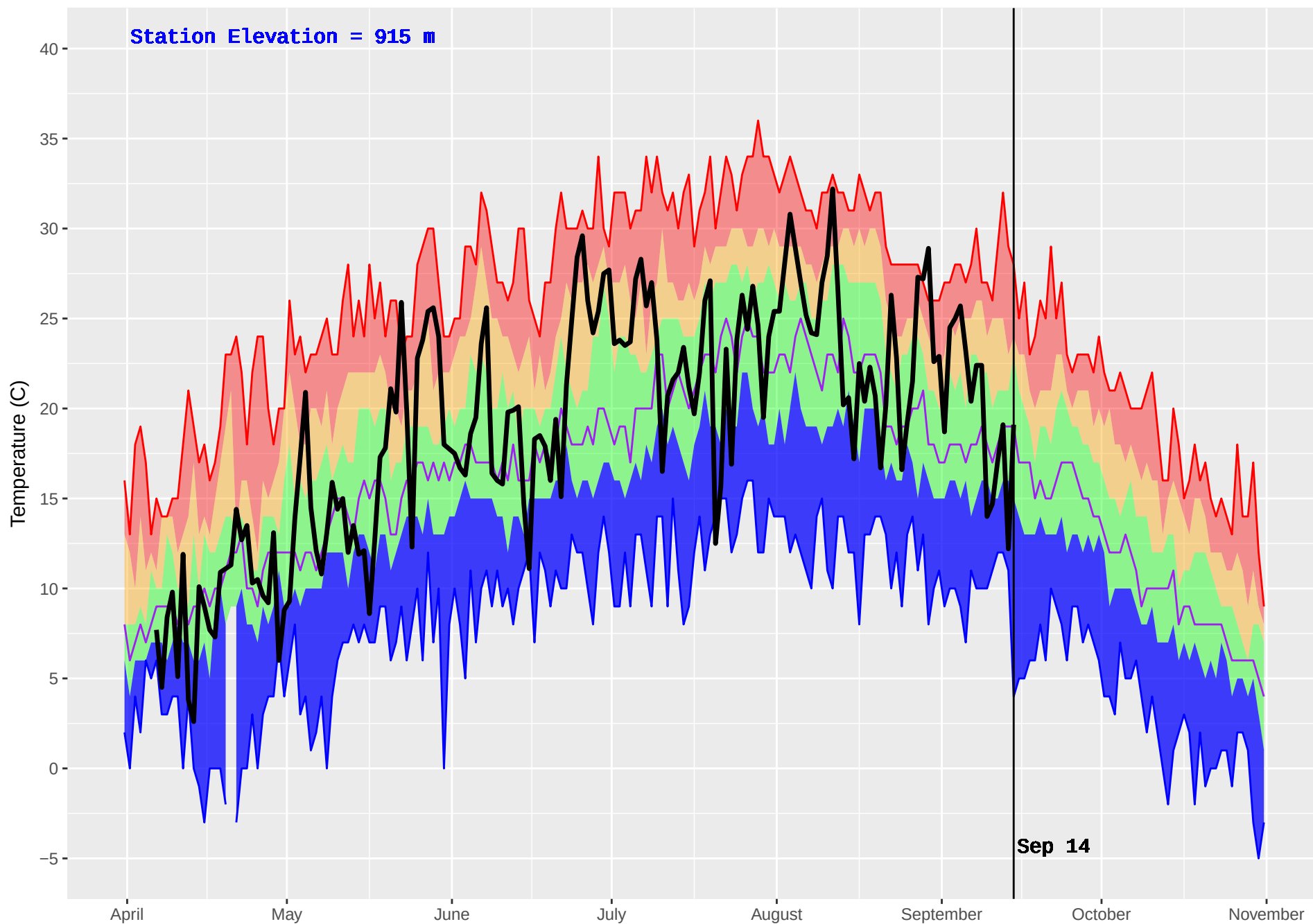
MIDDLE LAKE (226) : Historical (1989–2016) and Current (2017) Noon Temperature
