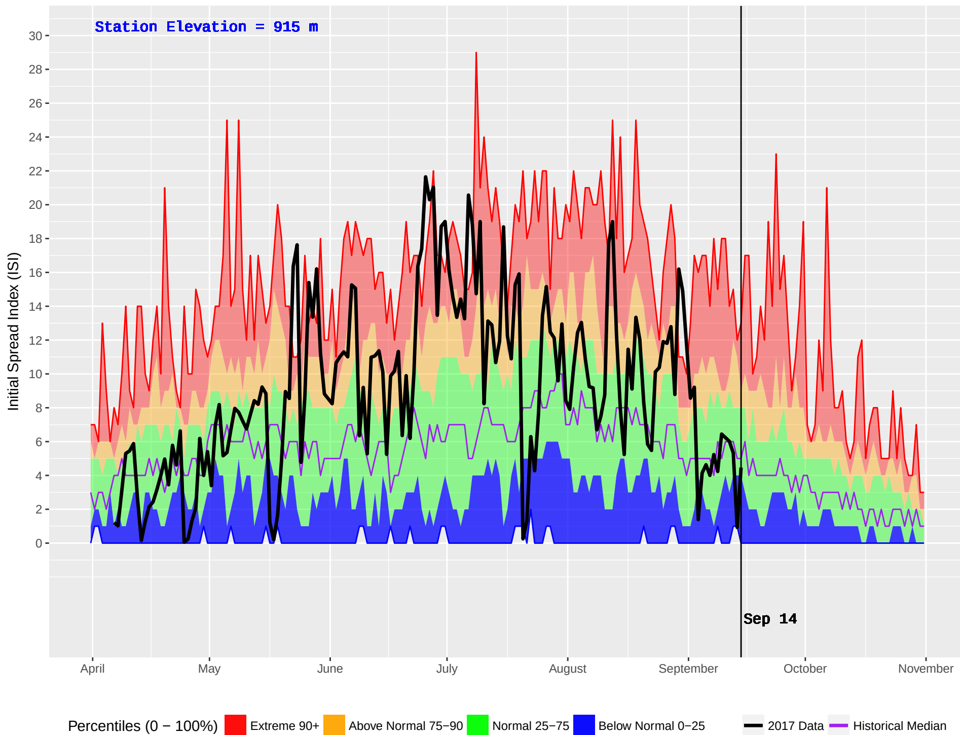
MIDDLE LAKE (226) : Historical (1989–2016) and Current (2017) Noon Initial Spread Index (ISI)
