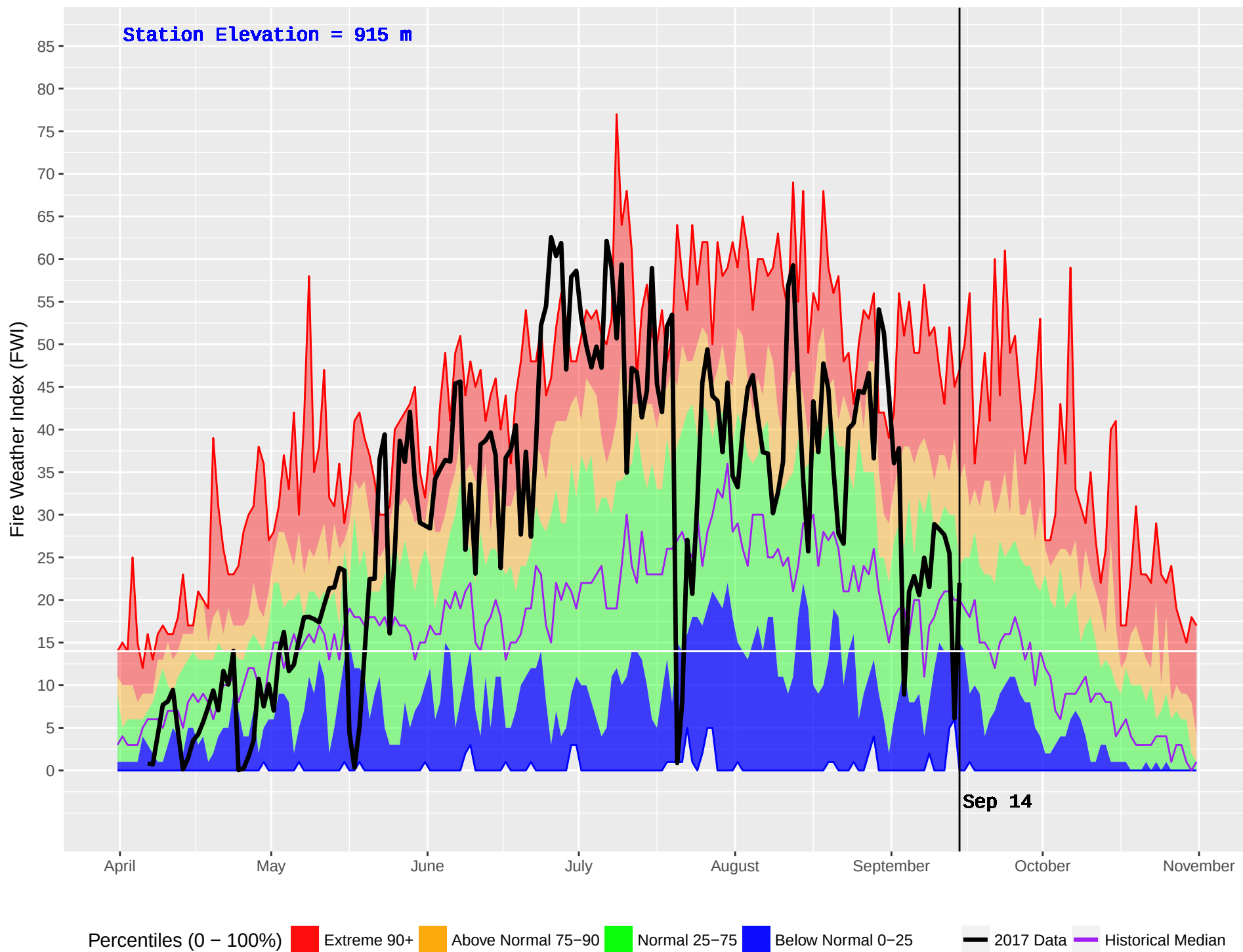
MIDDLE LAKE (226) : Historical (1989–2016) and Current (2017) Noon Fire Weather Index (FWI)
